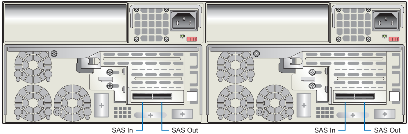
ContentServer 3160 - Rear panel view showing external SAS connectivity
