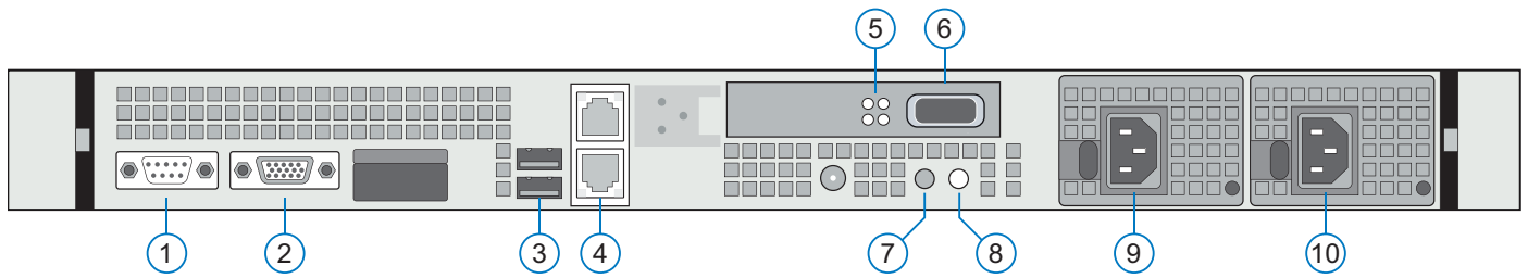
High Bandwidth ContentBridge - Rear Panel View
