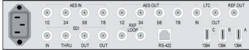
MediaPort 1010a - Rear Panel View
